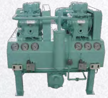
Water Cooled Provision Refrigeration Plant
